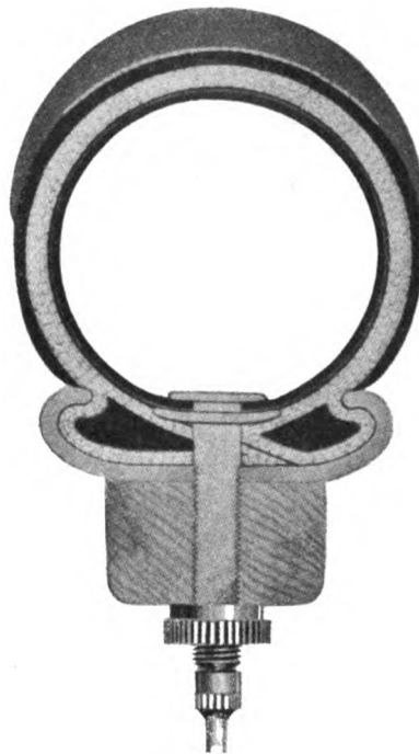
CROSS SECTION GENESEETIRE.
